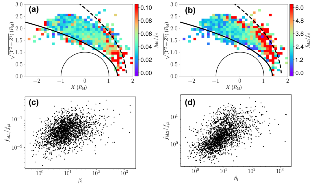
Figure 7. Break-point shifts of the plateau-like spectra. (a–b) Statistical maps of the normalized break-point frequencies f_{bk1}/f_{\rho} and f_{bk2}/f_{\rho} . (c) f_{bk1}/f_{\rho} as a function of local \beta_i . (d) f_{bk2}/f_{\rho} as a function of local \beta_i .
