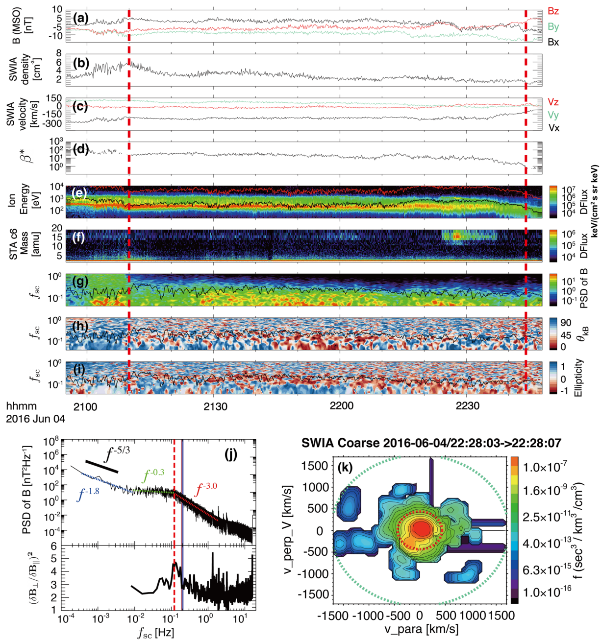
Figure 1. Mars Atmosphere and Volatile EvolutionN observations of the Martian magnetosheath crossing event on 4 June 2016. The magnetosheath interval is denoted by two vertical dashed lines in red. (a) Magnetic field in MSO coordinates from MAG. (b) Number density of ions from Solar Wind Ion Analyzer (SWIA). (c) Bulk velocity of ions in MSO coordinates from SWIA. (d) \beta^* . (e) Differential energy flux spectrogram of ions from SWIA. The maximum energy of pickup O^+ and H^+ are denoted by the lines in red and black. (f) Mass spectrogram of ions from STATIC. (g) Power spectral density spectrogram of the magnetic field. (h) Wave normal angle \theta_{kB} . (i) Ellipticity. The black lines in (g, h, and i) represent the Doppler-shifted proton cyclotron frequency. (j) PSD of the magnetic field within the magnetosheath interval. Vertical lines denote the characteristic ion-scale frequencies f_{pi} (light red), f_{di} (light blue), and f_{bk2} (red dashed line). (k) Velocity distribution function of the ions in the plane of (v_{\parallel}, v_{\perp}) retrieved from SWIA data from 22:28:03 to 22:28:07. The dotted circles represent the maximum pickup energy of H^+ (red) and O^+ (green).
